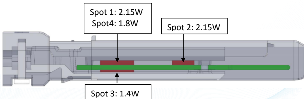
Figure 10: ML4022-LB-7.5W Power Spots Location
